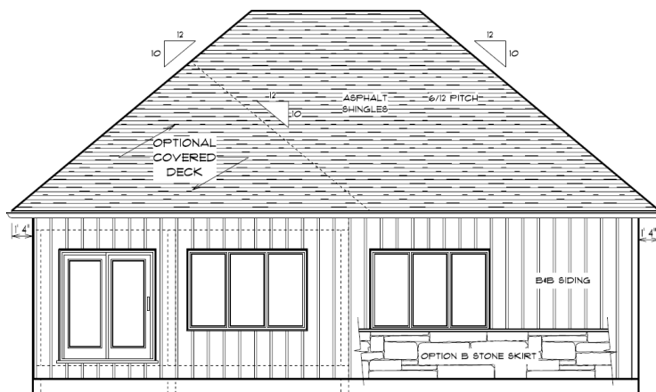
Rear Elevation
