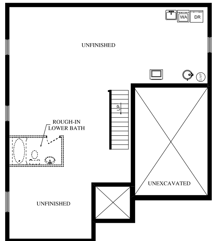
FOUNDATION PLAN
